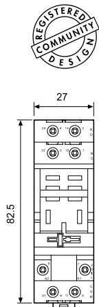
96.02
