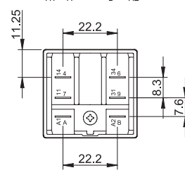
62.32-4800
